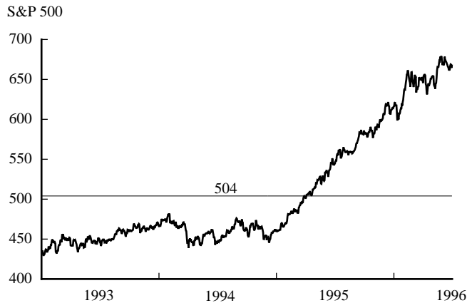
Chart 4.5 Observed nonstationary time series S&P 500 index
