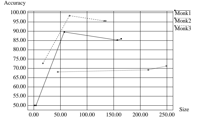
Figure 3: Complexity vs. Accuracy
