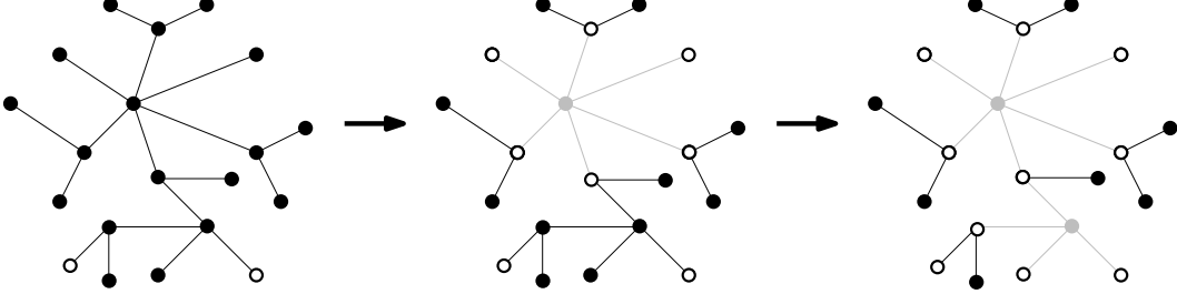
■ Figure 1 Schematic depiction of a single step of our centroid decomposition. After removing the grayed out node and its adjacent edges we obtain 6 pieces. One of them contains three boundary nodes and hence needs to be further partitioned into 4 smaller pieces.
